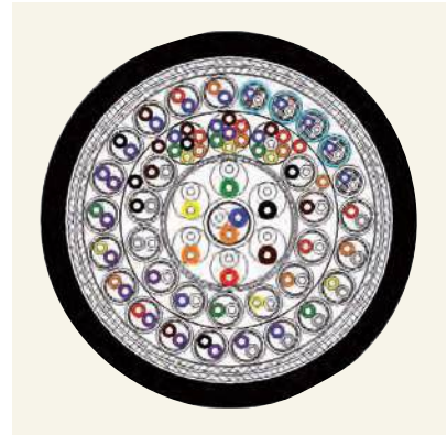
COMPOSITE ROUND CABLE
